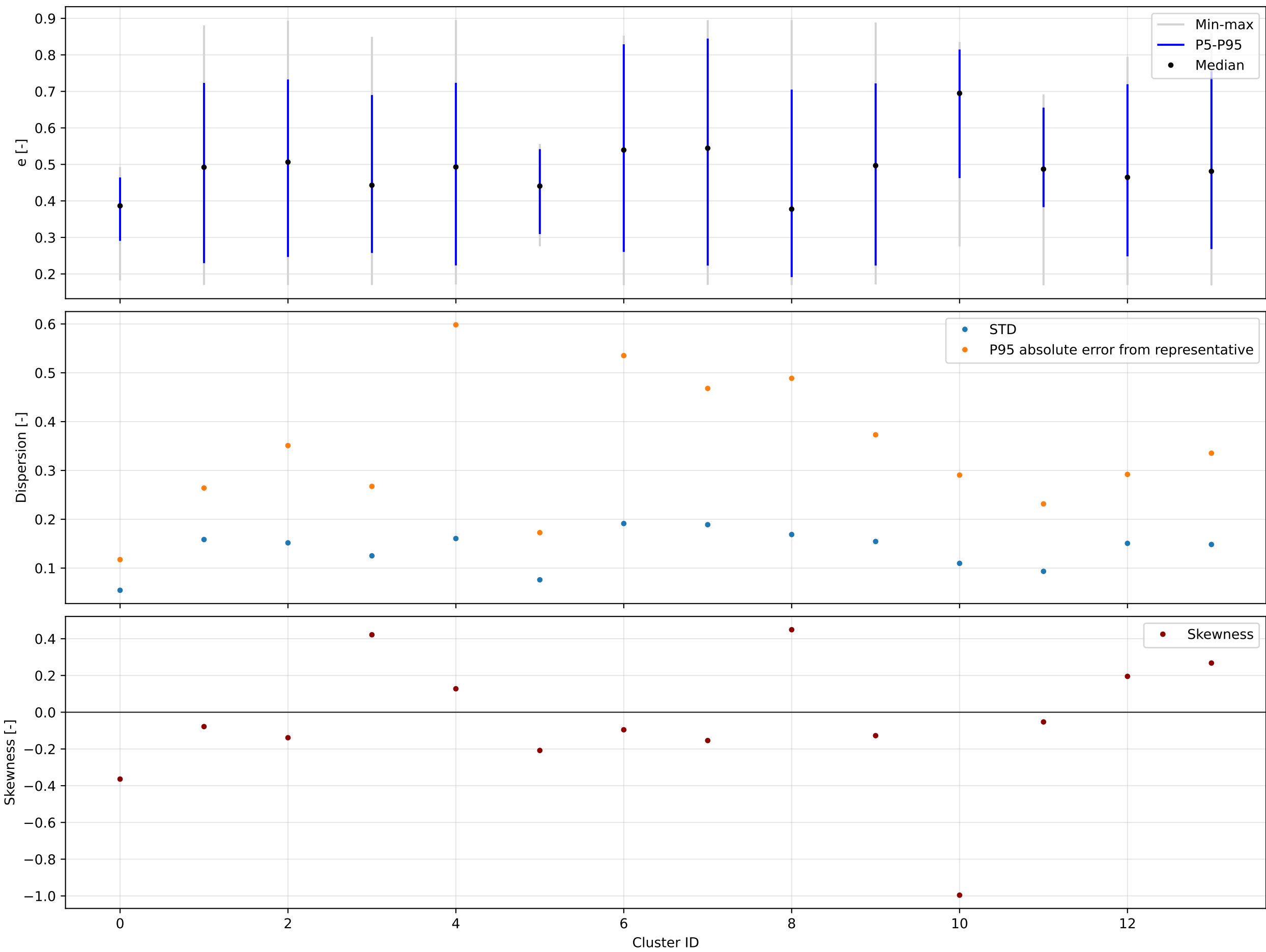
K=14 | forward | e | valid=194058/194058
