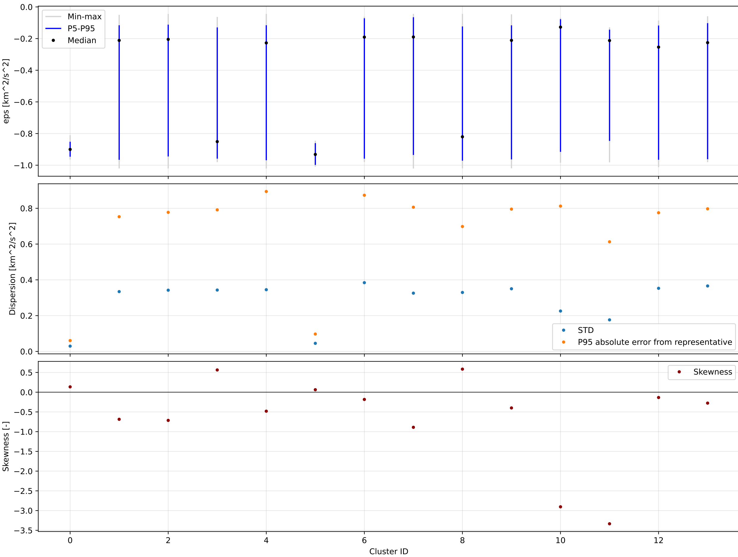
K=14 | forward | eps | valid=194058/194058
