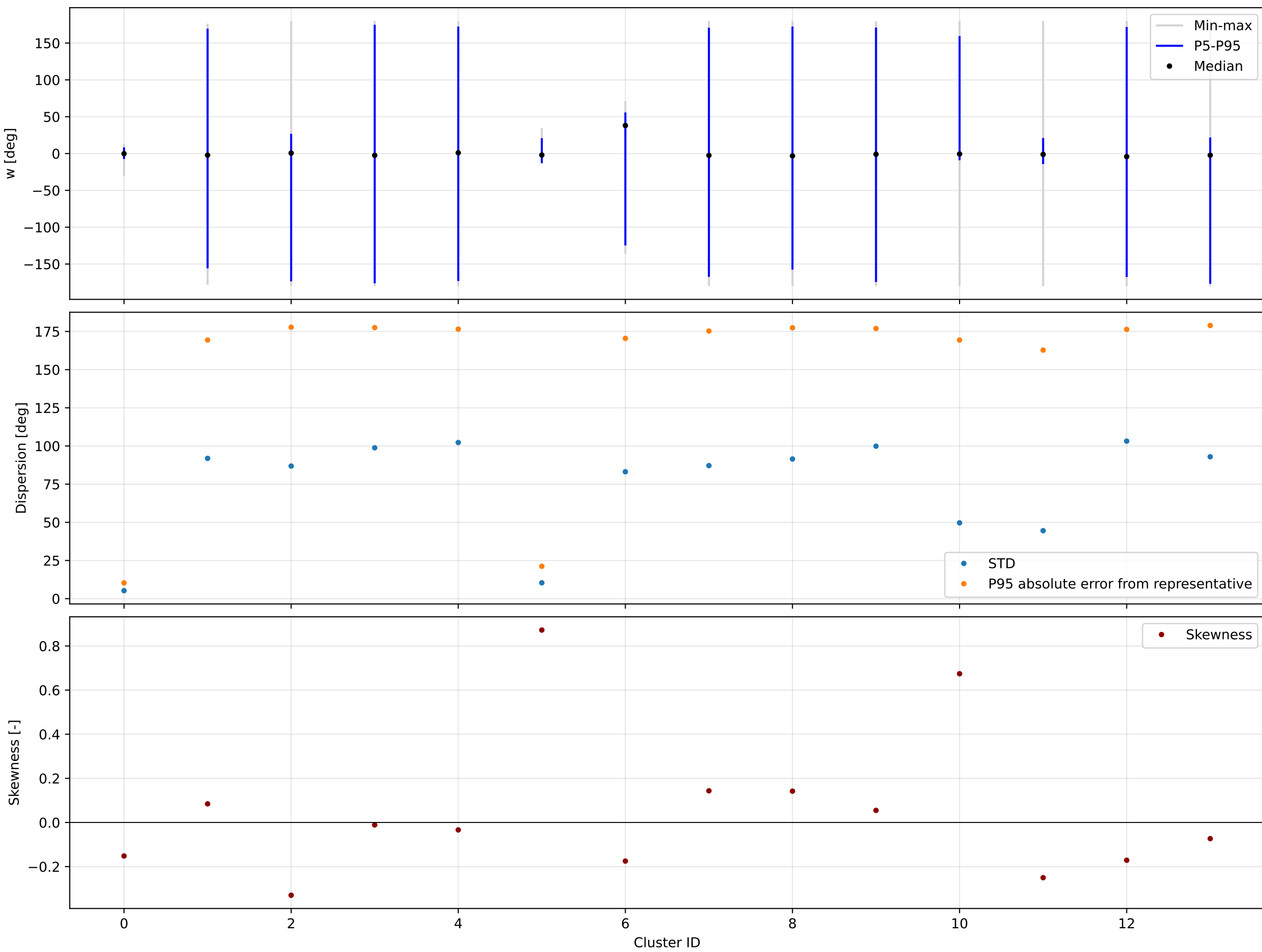
K=14 | forward | w | valid=194058/194058 | offsets from each cluster circular mean
