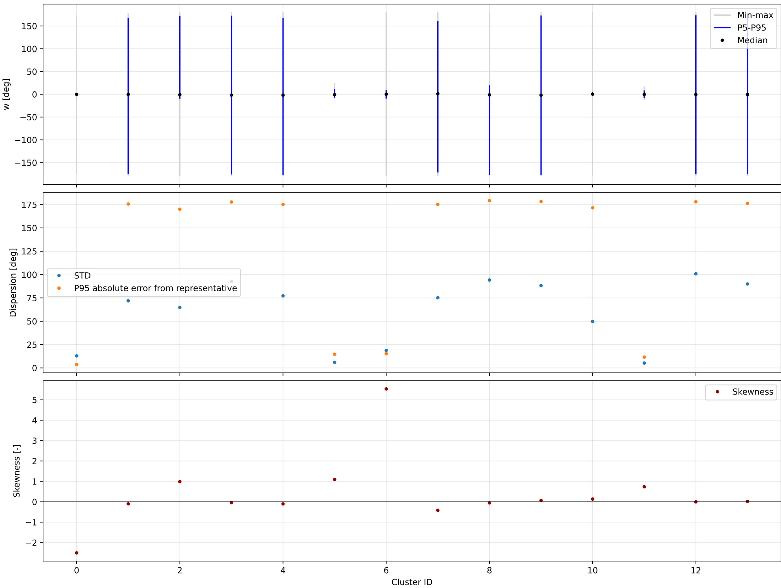
K=14 | backward | w | valid=194058/194058 | offsets from each cluster circular mean
